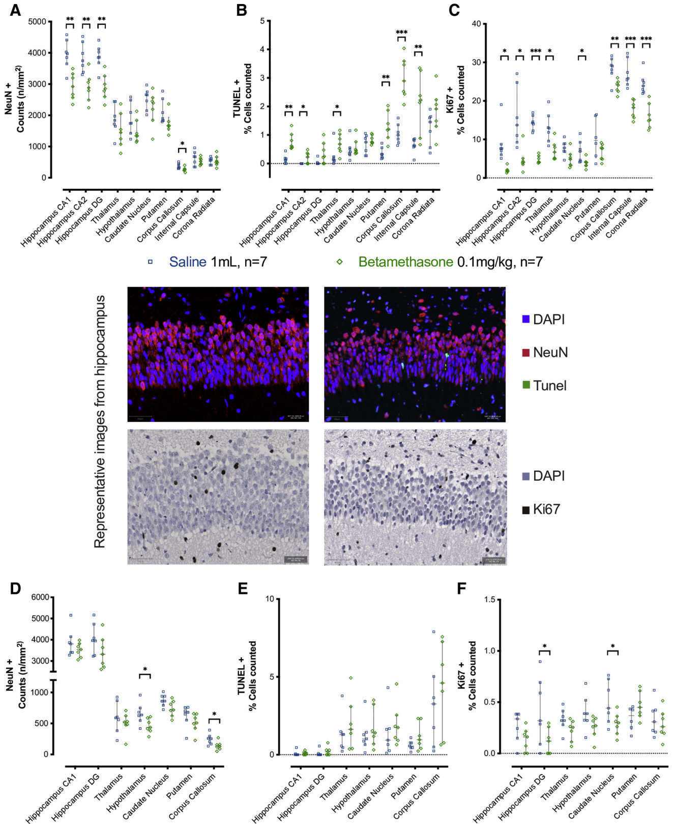
FIGURE 3 Neuropathological outcomes
