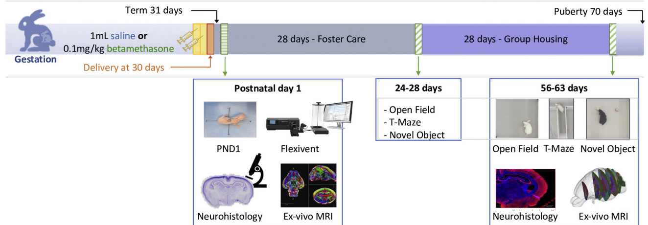
FIGURE 1 Study setup
