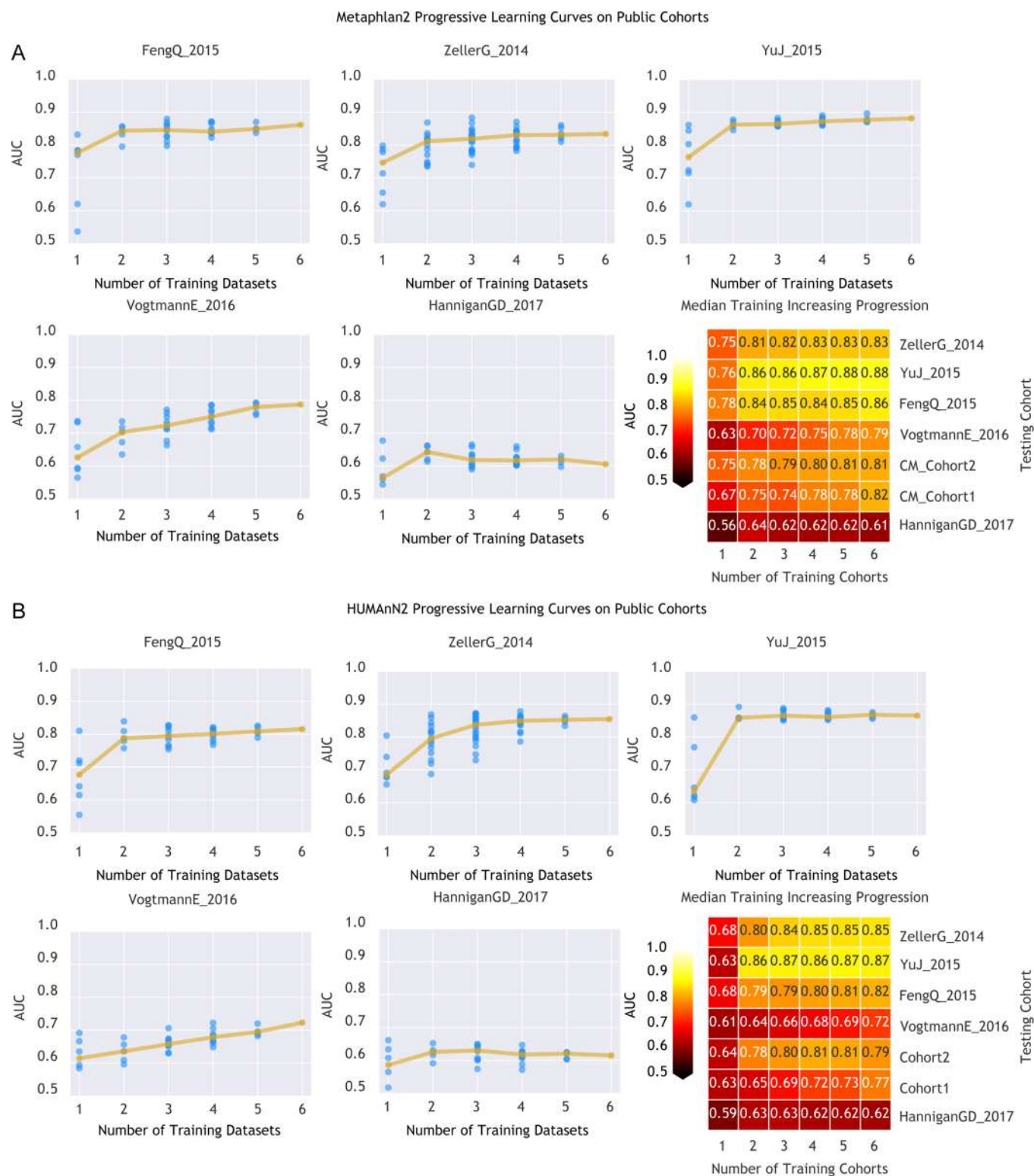
Extended Data Fig. 7 | Prediction performances with increasing numbers of external datasets considered in the training model. a, Prediction performances computed based on MetaPhlan2 species abundances. The dark yellow line interpolates the median AUC at each number of training datasets considered. b, Prediction performances computed based on HUMANn2 gene-family abundances.
